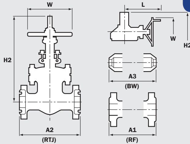
CLASS 150 - Bolted Bonnet Gate Valves
